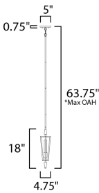
*max overall height
